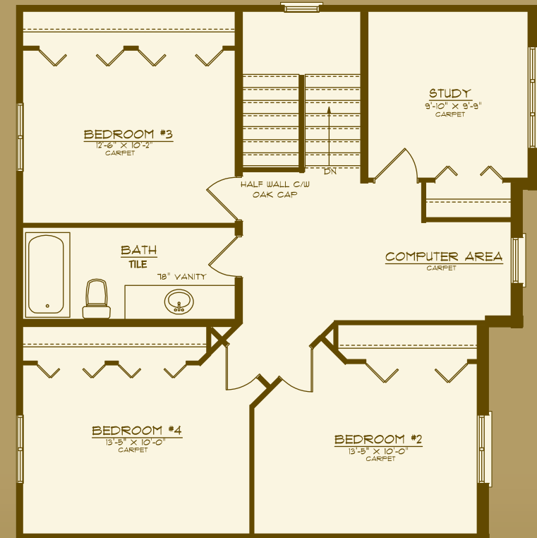
Upper Floor 932 Sq. Ft.
